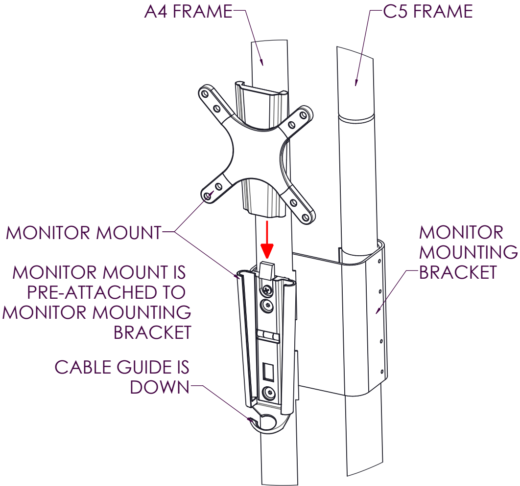
MONITOR MOUNT ATTACHMENT DETAIL ( MONITOR MOUNT IS OPTIONAL )
